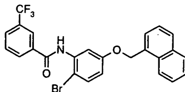
Compound # 34
